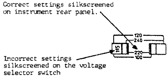
Figure 1. AC Line Voltage Switch Positions
